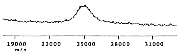
Fig. 4. Time of Flight mass spectra of AMDase and its complex with BPA. Positive ion was detected in each spectrum. a) Mass spectrum of native AMDase. Calculated value is 24734. b) Mass spectrum of AMDase after incubation with BPA.
